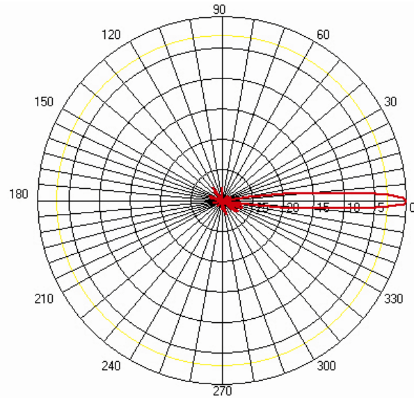
HPlane – Horizontal/Azimuth
