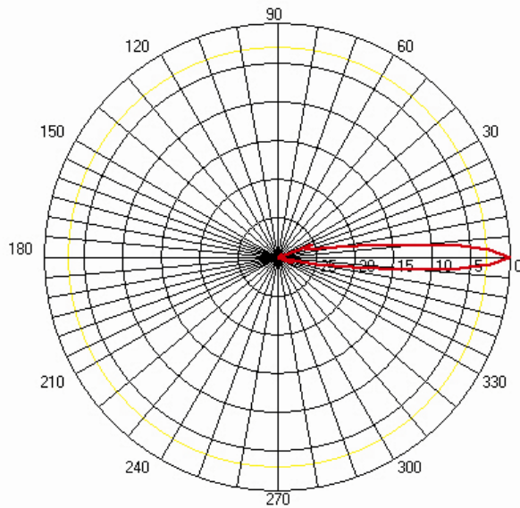
EPlane – Vertical/Elevation
